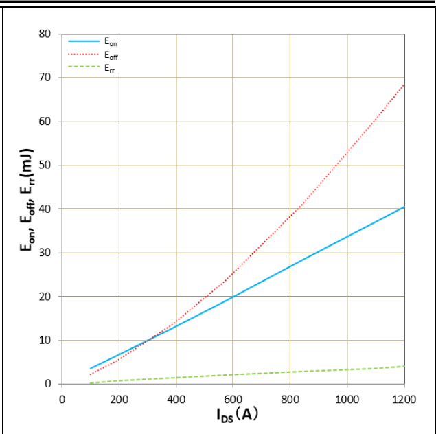
Figure 17. E_{on} , E_{off} , E_{rr} vs I_{DS} T_j = 150^\circ\text{C} , V_{DD} = 600\text{V} , R_G = 5.1\Omega , V_{GS} = +18\text{V}/-5\text{V} Inductive Load
