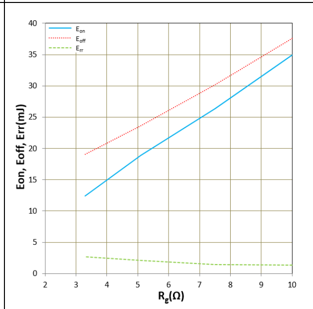
Figure 15. E_{on} , E_{off} , E_{rr} vs R_g T_j = 150^\circ\text{C} , V_{DD} = 600\text{V} , I_D = 600\text{A} , V_{GS} = +18\text{V}/-5\text{V} Inductive Load
