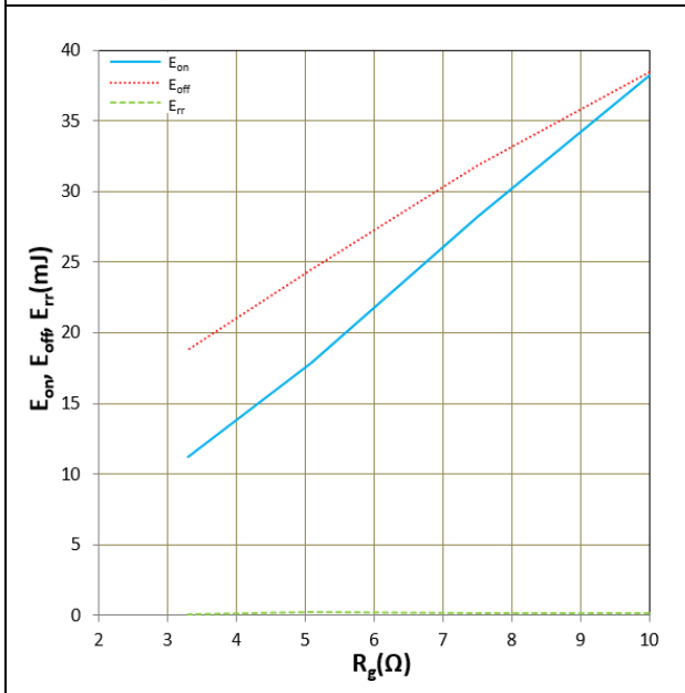
Figure 14. E_{on} , E_{off} , E_{rr} vs R_g T_j = 25^\circ\text{C} , V_{DD} = 600\text{V} , I_D = 600\text{A} , V_{GS} = +18\text{V}/-5\text{V} Inductive Load
