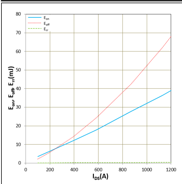
Figure 16. E_{on} , E_{off} , E_{rr} vs I_{DS} T_j = 25^\circ\text{C} , V_{DD} = 600\text{V} , R_G = 5.1\Omega , V_{GS} = +18\text{V}/-5\text{V} Inductive Load
