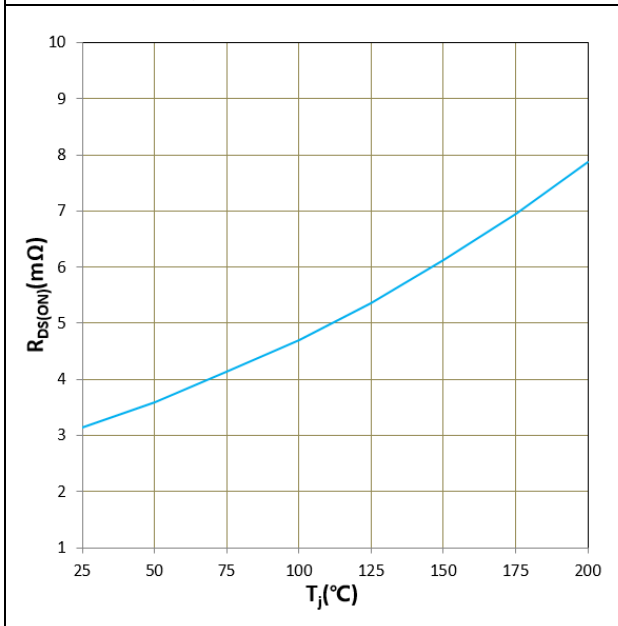
Figure 10. R_{DS(ON)} vs T_j V_{GS} = +18\text{V} , I_D = 400\text{A}
