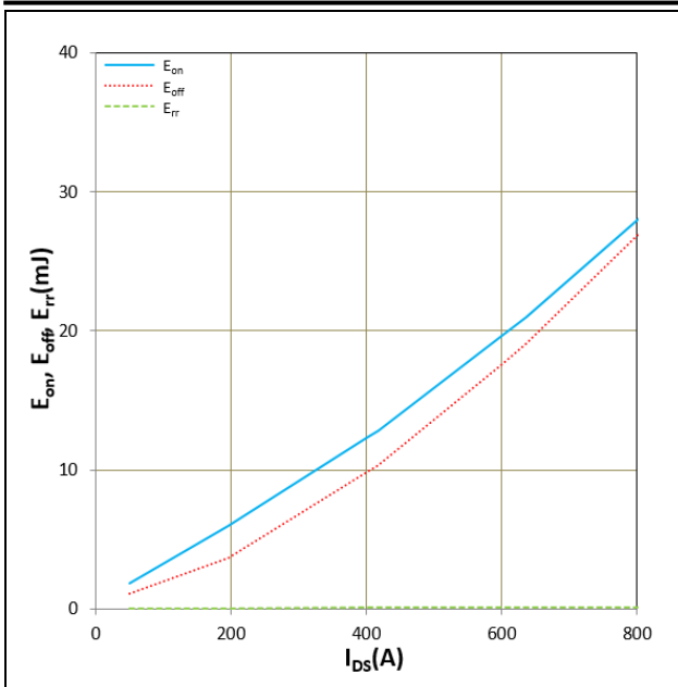
Figure 16. E_{on} , E_{off} , E_{rr} vs I_{DS} T_j = 25^\circ\text{C} , V_{DD} = 600\text{V} , R_g = 5.6\Omega , V_{GS} = +18\text{V}/-5\text{V} Inductive Load
