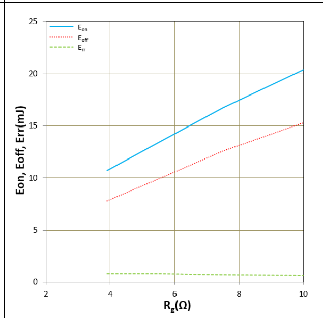
Figure 15. E_{on} , E_{off} , E_{rr} vs R_g T_j = 150^\circ\text{C} , V_{DD} = 600\text{V} , I_D = 400\text{A} , V_{GS} = +18\text{V}/-5\text{V} Inductive Load
