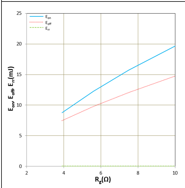
Figure 14. E_{on} , E_{off} , E_{rr} vs R_g T_j = 25^\circ\text{C} , V_{DD} = 600\text{V} , I_D = 400\text{A} , V_{GS} = +18\text{V}/-5\text{V} Inductive Load
