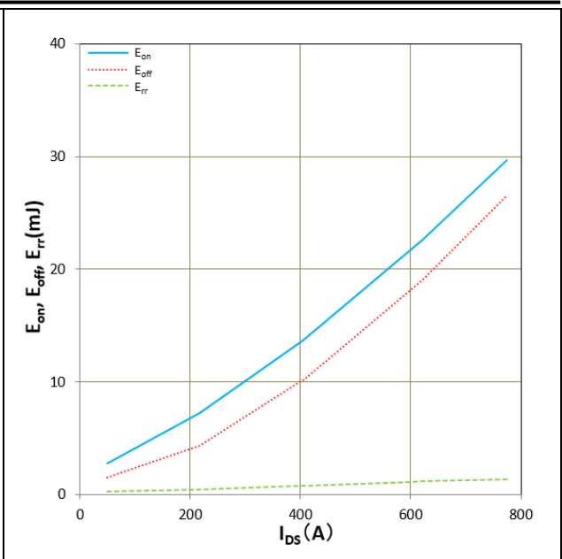
Figure 17. E_{on} , E_{off} , E_{rr} vs I_{DS} T_j = 150^\circ\text{C} , V_{DD} = 600\text{V} , R_g = 5.6\Omega , V_{GS} = +18\text{V}/-5\text{V} Inductive Load
