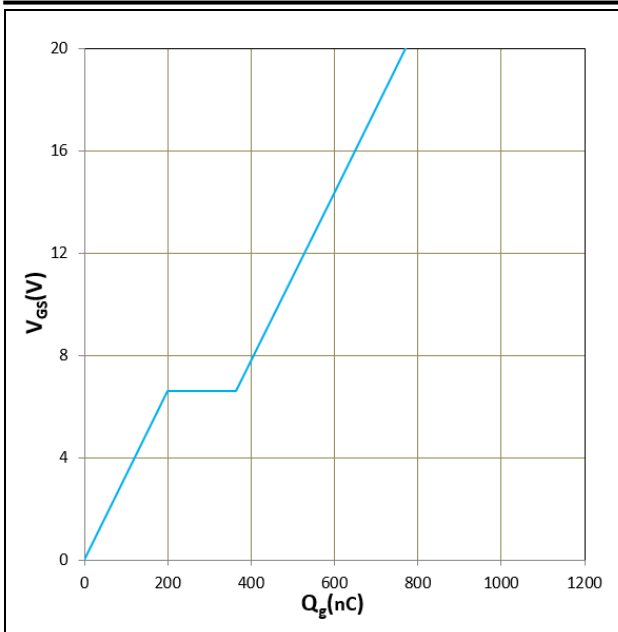
Figure 12. V_{GS} vs Q_g T_j = 25^\circ\text{C} , I_D = 250\text{A} , V_{DS} = 920\text{V}
