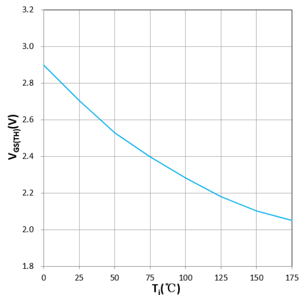
Figure 12. V_{GS(TH)} vs T_j V_{GS} = V_{DS} , I_D = 70mA
