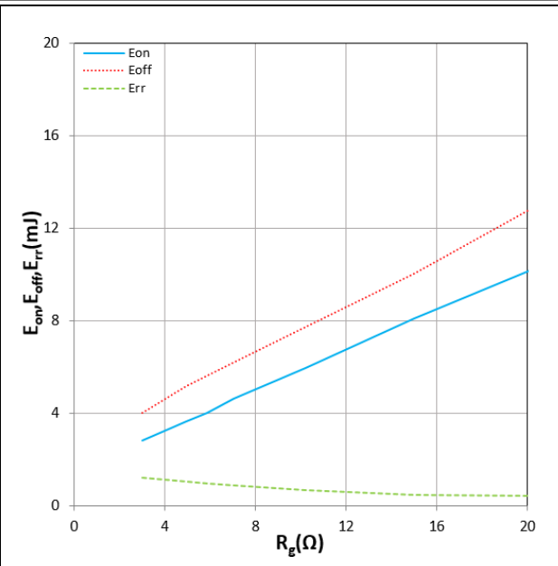
Figure 14. E_{on} , E_{off} , E_{rr} vs R_g T_j = 150^\circ\text{C} , V_{DD} = 600\text{V} , V_{GS} = +18\text{V}/-4\text{V} , I_D = 200\text{A} Inductive Load
