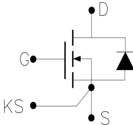
Figure 1. Out drawing & circuit diagram for DFS17SU12Z7C1
