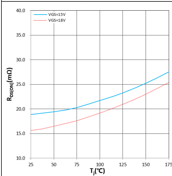
Figure 11. R_{DS(ON)} vs T_j I_D = 60\text{A}
