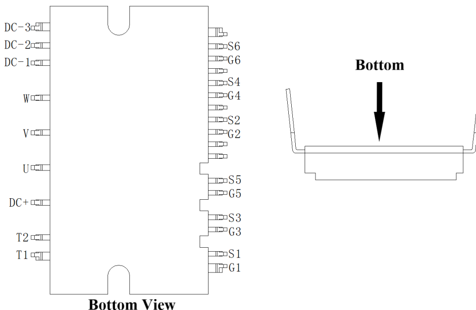
Figure 2. Pin configuration
