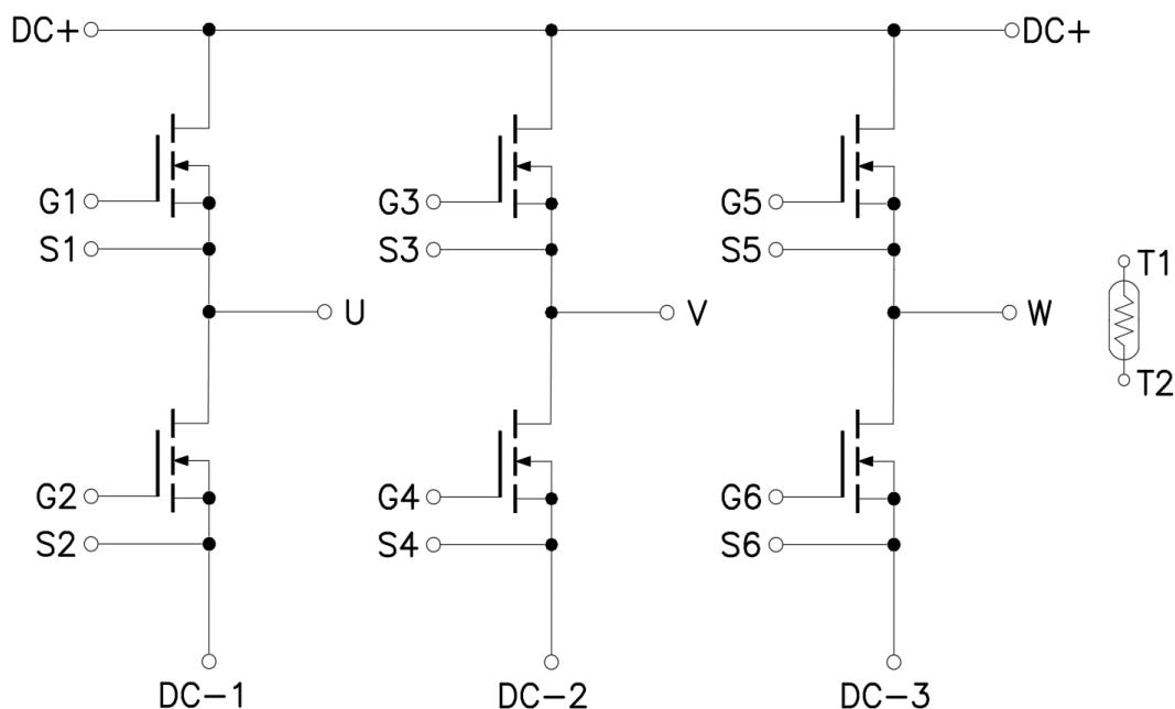
Figure 1. Out drawing & circuit diagram for DFS37FB12M6Q1
