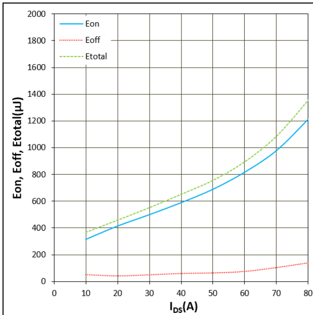
Figure 13. E_{on} , E_{off} , E_{total} vs I_D T_j = 150^\circ\text{C} , R_G = 2.5\Omega , V_{GS} = -5/+20\text{V}
