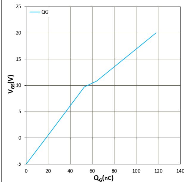
Figure 15. V_{GS} vs Q_G T_j = 25^\circ\text{C} , V_{DD} = 800\text{V} , I_D = 40\text{A}
