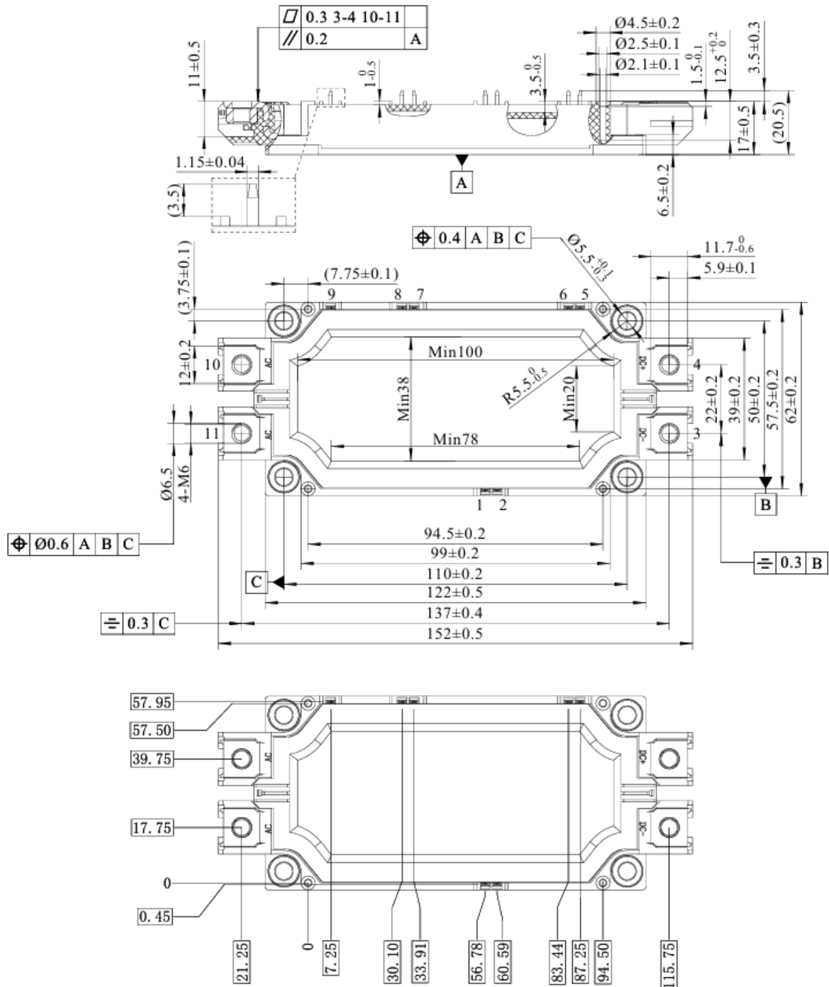
Figure 2. Pin configuration
