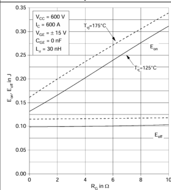
Figure 10. Typical switching energies per pulse vs. gate resistor
