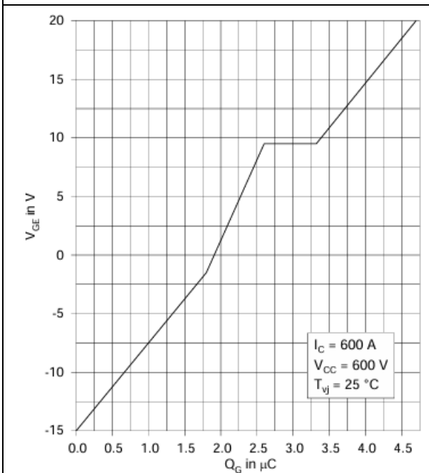
Figure 13. Typical gate charge characteristics
