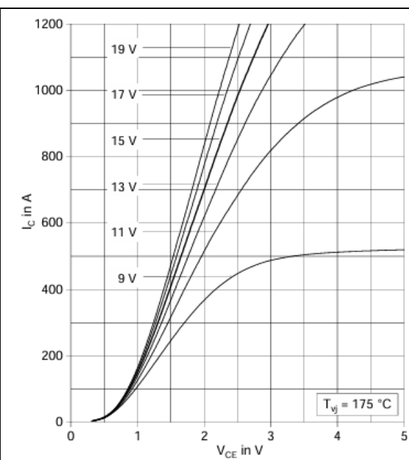
Figure 8. Typical output characteristics, chip level
