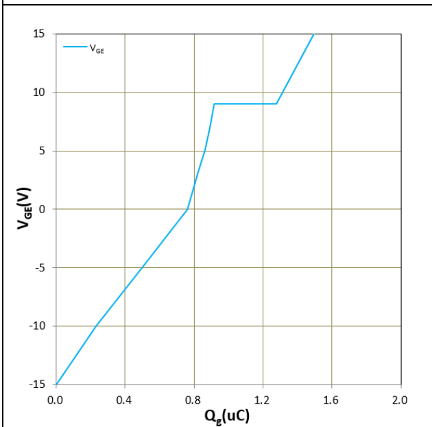
Figure 13. Gate charge
