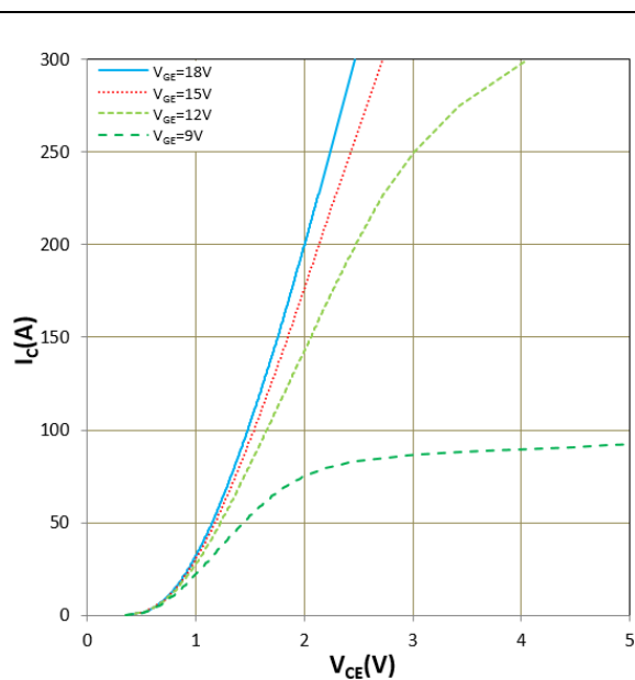
Figure 6. I_C vs V_{CE} T_j = 175^\circ C
