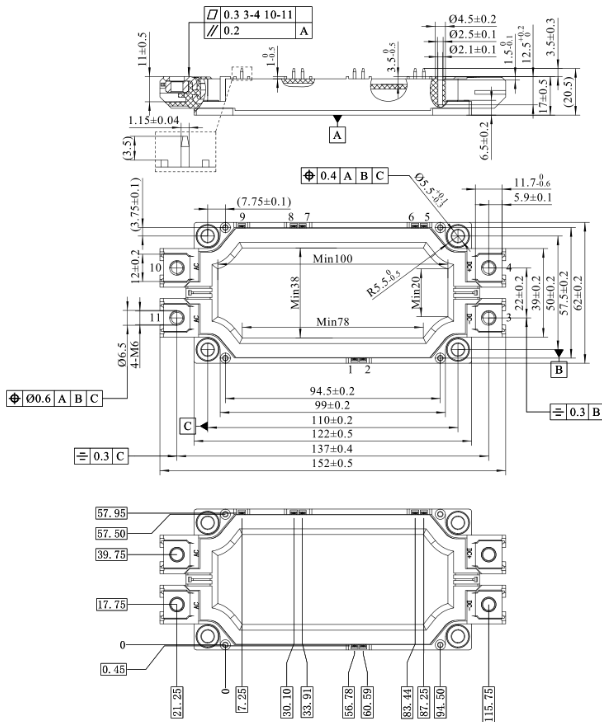
Figure 2. Pin configuration
