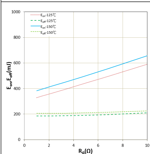
Figure 9. E_{on} , E_{off} vs R_G (Typ) V_{CC} = 900V , V_{GE} = +15V/-8V , I_c = 600A Inductive Load
