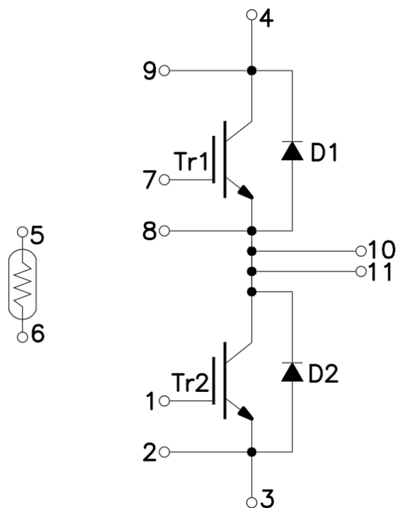
Figure 1. Out drawing & circuit diagram for DFI600HF17I4RE1PN
