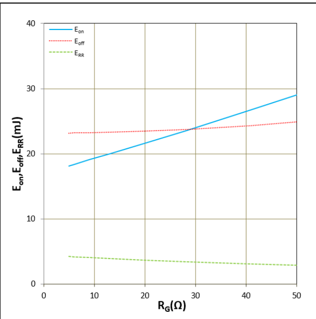
Figure 12. E_{on} , E_{off} vs R_G (Typ) V_{CC}=900V , V_{GE}=+15V/-8V , I_C=75A , T_j=150^\circ C Inductive Load
