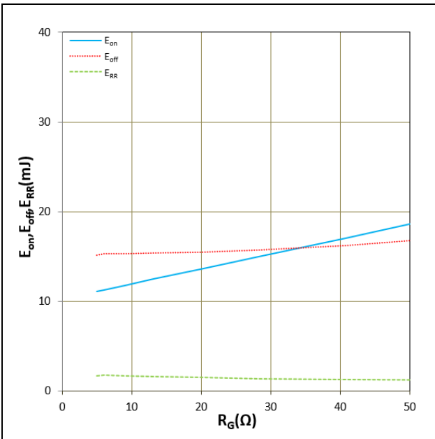
Figure 11. E_{on} , E_{off} vs R_G (Typ) V_{CC}=900V , V_{GE}=+15V/-8V , I_C=75A , T_j=25^\circ C Inductive Load
