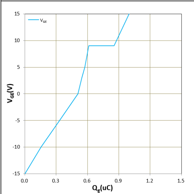
Figure 13. Gate charge
