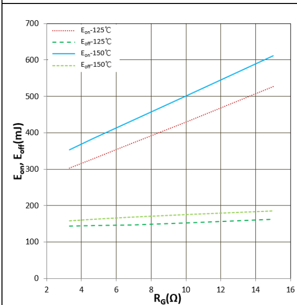
Figure 9. E_{on} , E_{off} vs R_g (Typ) V_{CC}=900V , V_{GE}=+15V/-8V , I_c=450A Inductive Load
