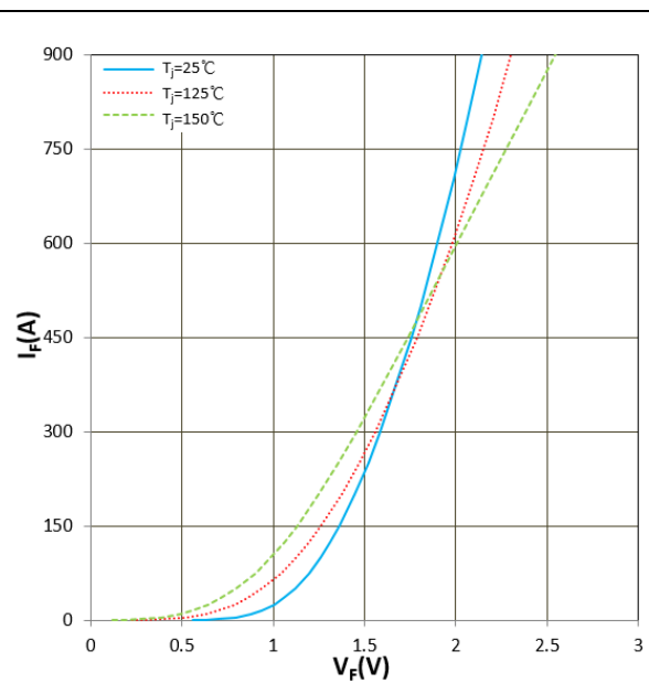
Figure 16. I_F vs V_F
