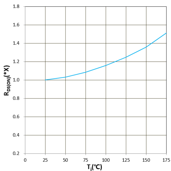
Figure 9. R DS(ON) vs T j V GS = +15V, I D = 200A, 1.0X = 4.7mΩ
