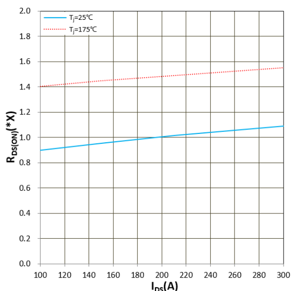
Figure 10. R DS(ON) vs I DS V GS = +15V, 1.0X = 4.7mΩ
