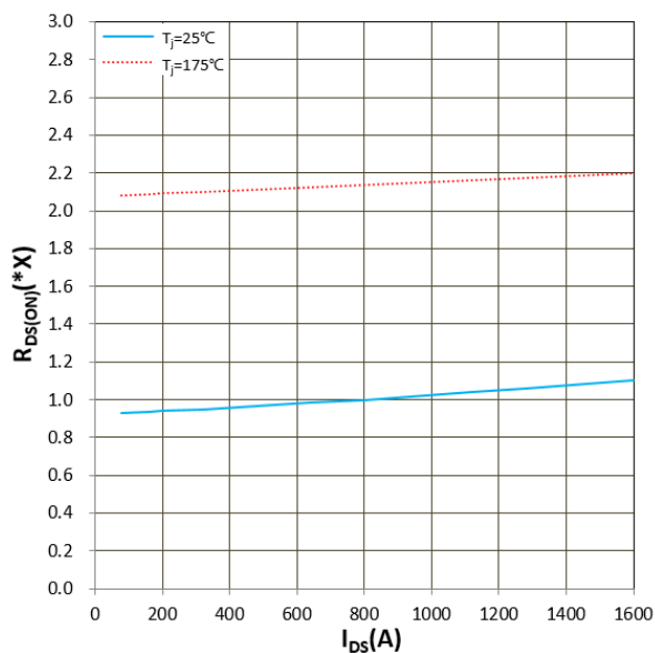
Figure 12. R_{DS(ON)} vs I_{DS} V_{GS} = +15V , 1.0x = 4.0m\Omega
