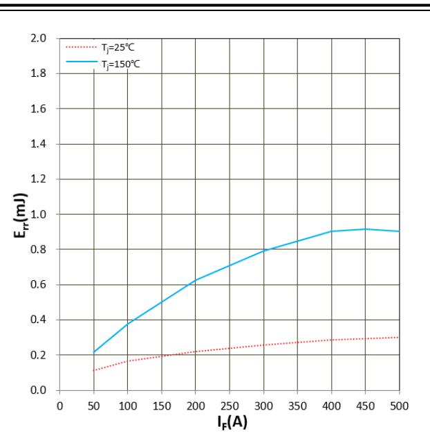
Figure 21. E_{rr} vs I_F V_{DD} = 600V , R_g = 10\Omega , V_{GS} = +15V/-4V Inductive Load
