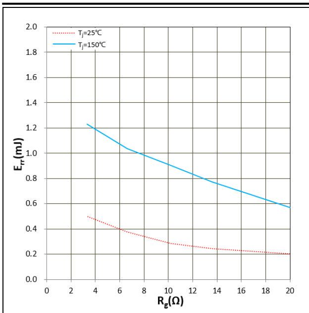
Figure 20. E_{rr} vs R_g V_{DD} = 600V , I_F = 400A , V_{GS} = +15V/-4V Inductive Load
