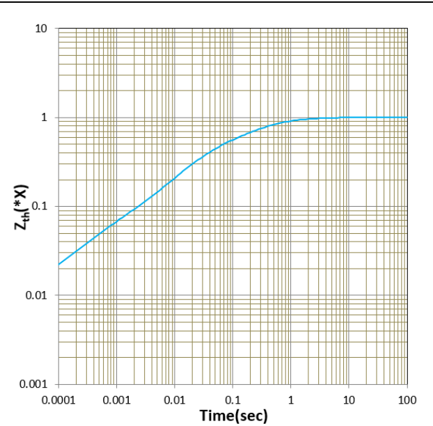
Figure 23. Transient thermal impedance 1.0x = 0.156K/W
