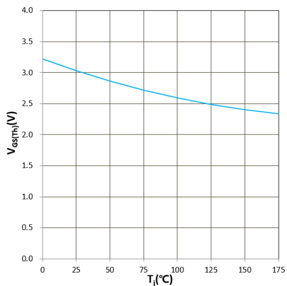
Figure 15. V_{GS(TH)} vs T_J V_{GS} = V_{DS} , I_D = 40mA
