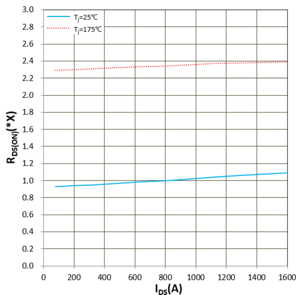
Figure 13. R_{DS(ON)} vs I_{DS} V_{GS} = +18V , 1.0x = 3.4m\Omega
