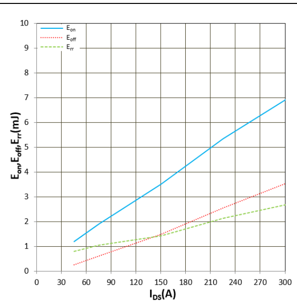
Figure 16. E_{on} , E_{off} , E_{rr} vs I_{DS} T_j = 150^\circ\text{C} , V_{CC} = 600\text{V} , R_G = 3.3\Omega , V_{GS} = -5\text{V}/+15\text{V} Inductive Load
