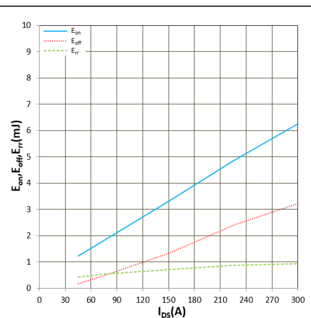
Figure 14. E_{on} , E_{off} , E_{rr} vs I_{DS} T_j = 25^\circ\text{C} , V_{CC} = 600\text{V} , R_G = 3.3\Omega , V_{GS} = -5\text{V}/+15\text{V} Inductive Load
