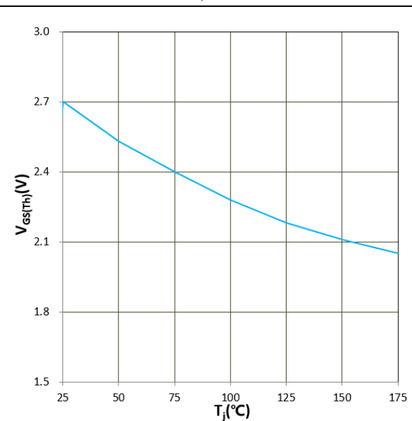
Figure 12. V GS(TH) vs T j V GS = V DS , I D = 105mA
