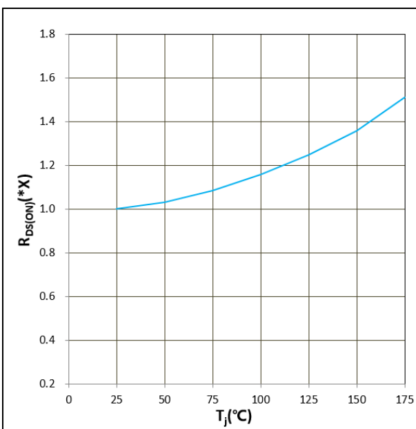
Figure 9. R DS(ON) vs T j V GS = +15V, I D = 200A, 1.0X = 6.5mΩ
