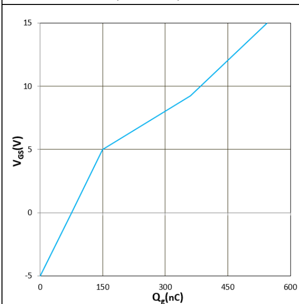
Figure 11. V GS vs Q g V DS = 800V, I D = 180A, T j = 25°C
