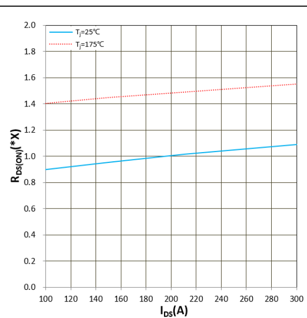
Figure 10. R DS(ON) vs I DS V GS = +15V, 1.0X = 6.5mΩ
