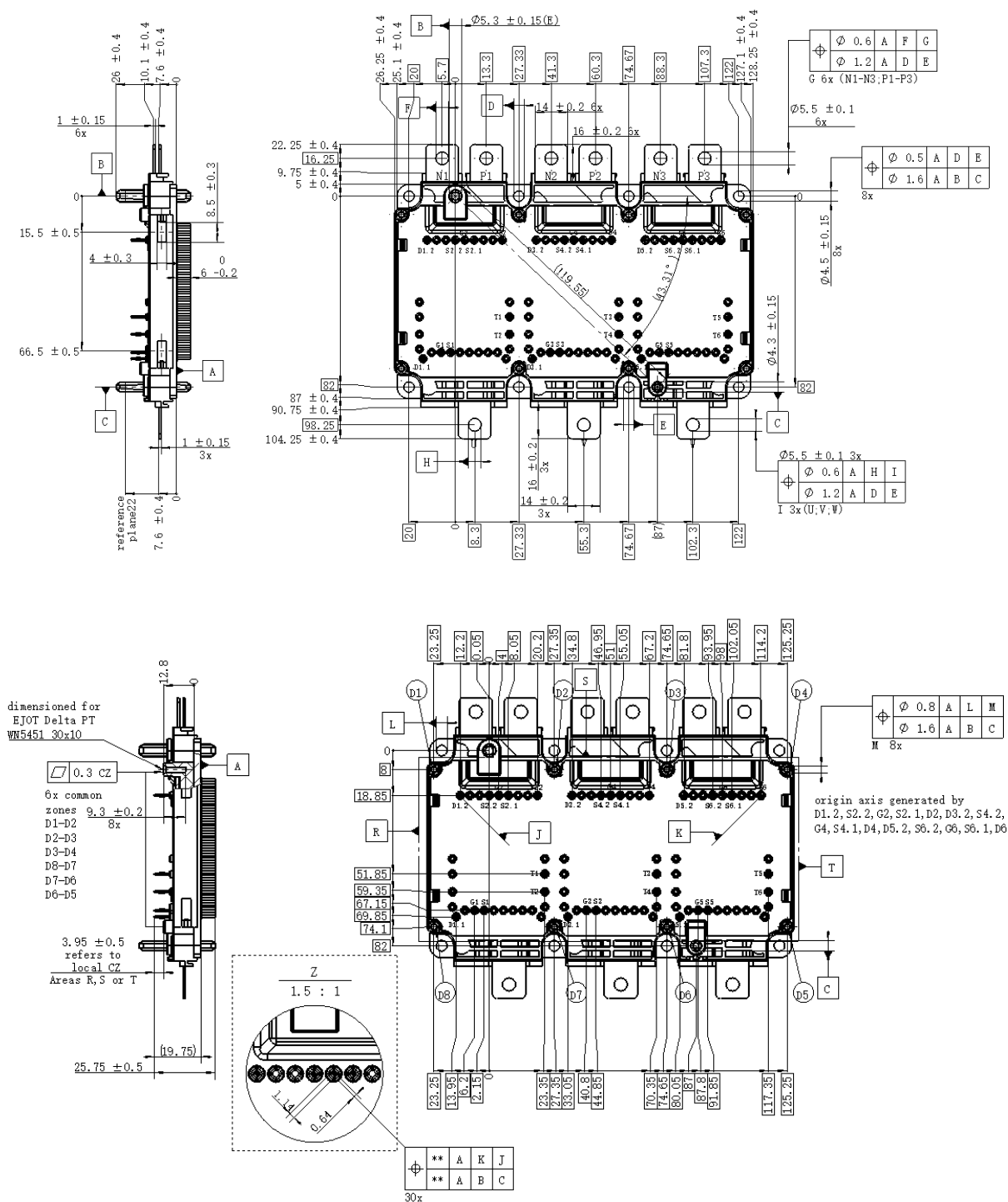
Figure2. Physical Dimensions
