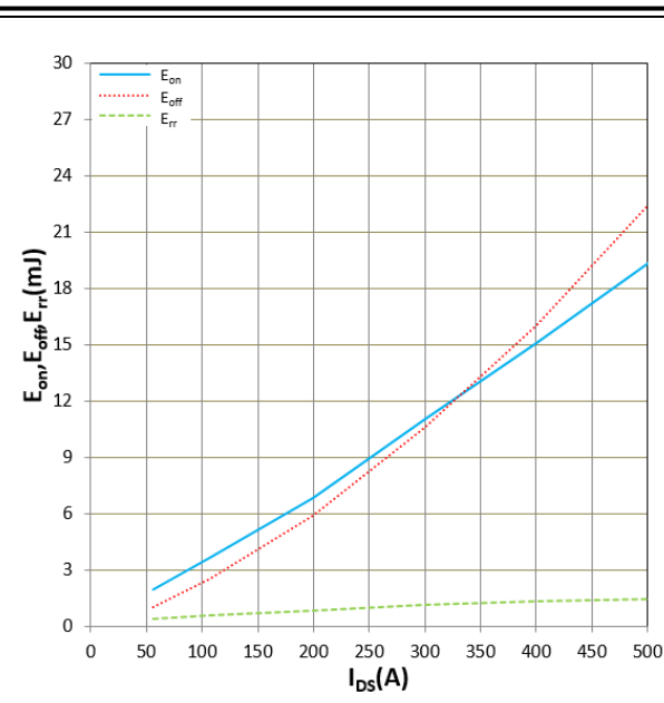
Figure 17. E_{on} , E_{off} , E_{rr} vs I_{DS} T_j = 150^\circ\text{C} , V_{CC} = 600\text{V} , R_G = 4.5\Omega , V_{GS} = +15\text{V}/-4\text{V} Inductive Load
