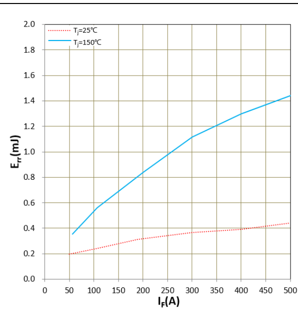
Figure 19. E_{rr} vs I_F V_{DD} = 600\text{V} , R_G = 4.5\Omega , V_{GS} = +15\text{V}/-4\text{V} Inductive Load
