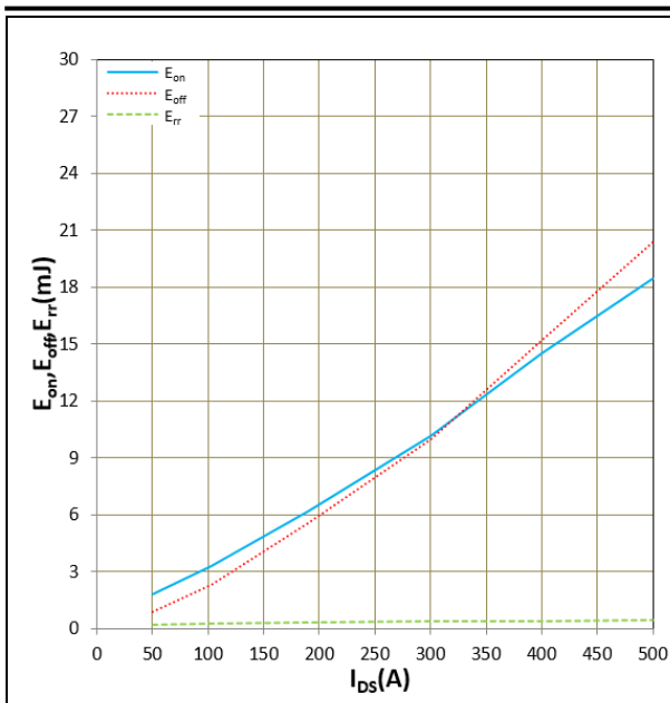
Figure 16. E_{on} , E_{off} , E_{rr} vs I_{DS} T_j = 25^\circ\text{C} , V_{CC} = 600\text{V} , R_G = 4.5\Omega , V_{GS} = +15\text{V}/-4\text{V} Inductive Load
