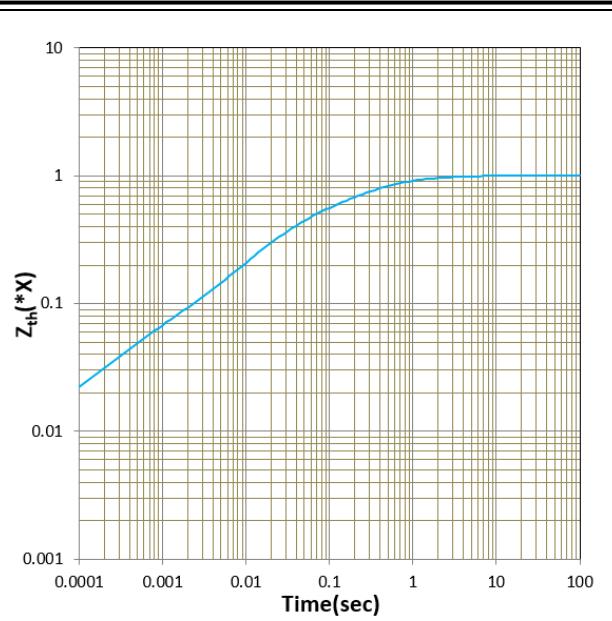
Figure 21. Transient thermal impedance 1.0x = 0.156K/W
