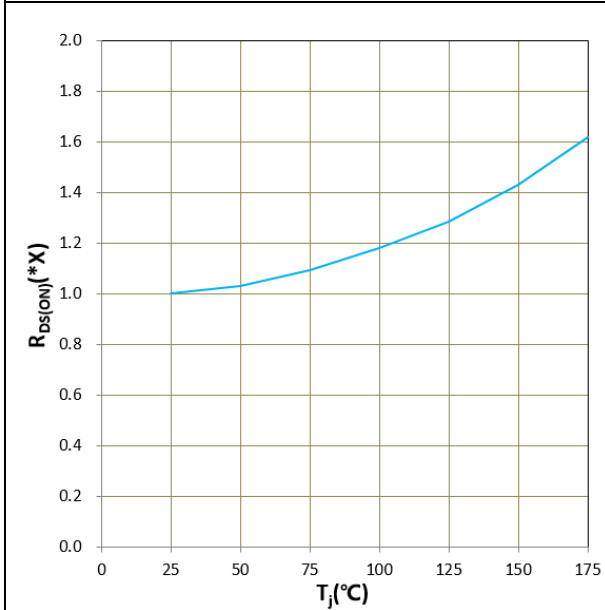
Figure 10. R_{DS(ON)} vs T_j 1.0x = 4.2m \Omega , I_D = 400\text{A}
