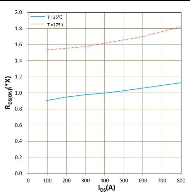
Figure 11. R_{DS(ON)} vs I_{DS} 1.0x = 4.2m \Omega
