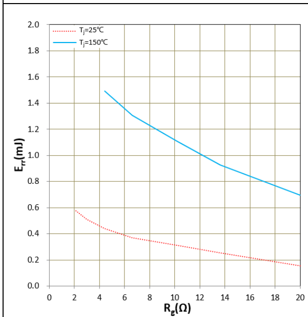
Figure 18. E_{rr} vs R_G V_{DD} = 600\text{V} , I_F = 400\text{A} , V_{GS} = +15\text{V}/-4\text{V} Inductive Load
