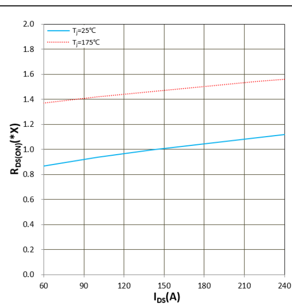
Figure 10. R DS(ON) vs I DS V GS = +15V, 1.0X = 10.1mΩ
