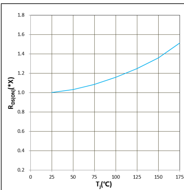
Figure 9. R DS(ON) vs T j V GS = +15V, I D = 150A, 1.0X = 10.1mΩ
