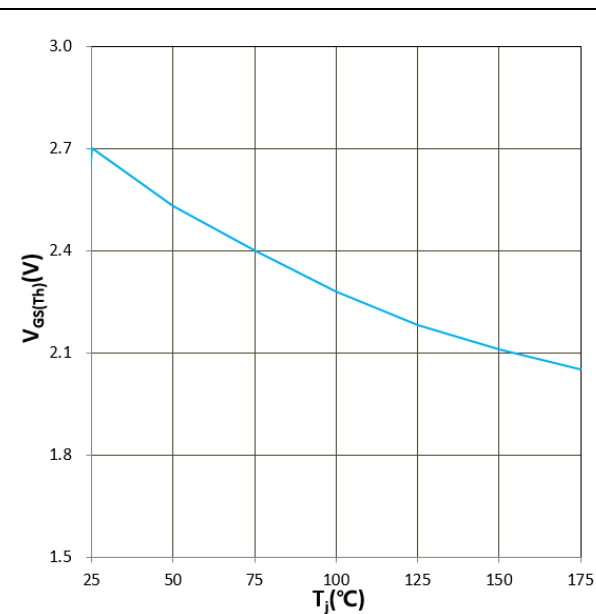
Figure 12. V GS(TH) vs T j V GS = V DS , I D = 70mA
