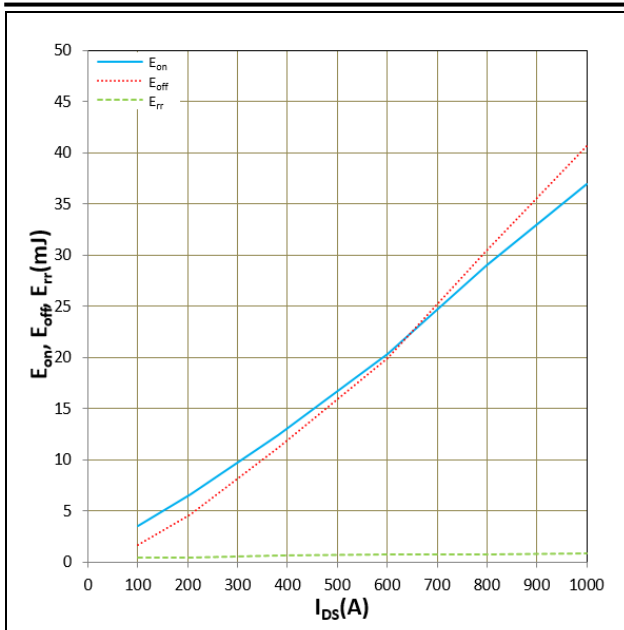
Figure 16. E on , E off , E rr vs I DS T j =25°C, V CC =600V, R G =2.2Ω, V GS =+15V/-4V Inductive Load
