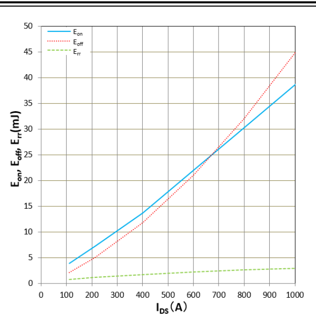
Figure 17. E on , E off , E rr vs I DS T j =150°C, V CC =600V, R G =2.2Ω, V GS =+15V/-4V Inductive Load
