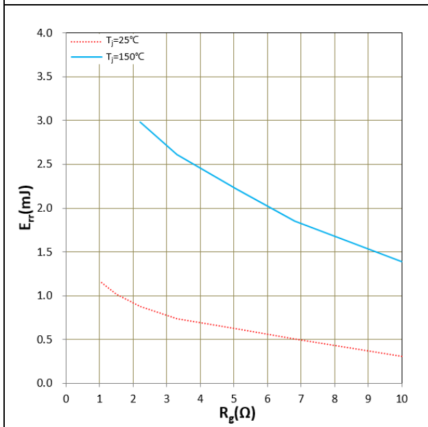
Figure 18. E rr vs R G V DD =600V, I F =800A, V GS =+15V/-4V Inductive Load
