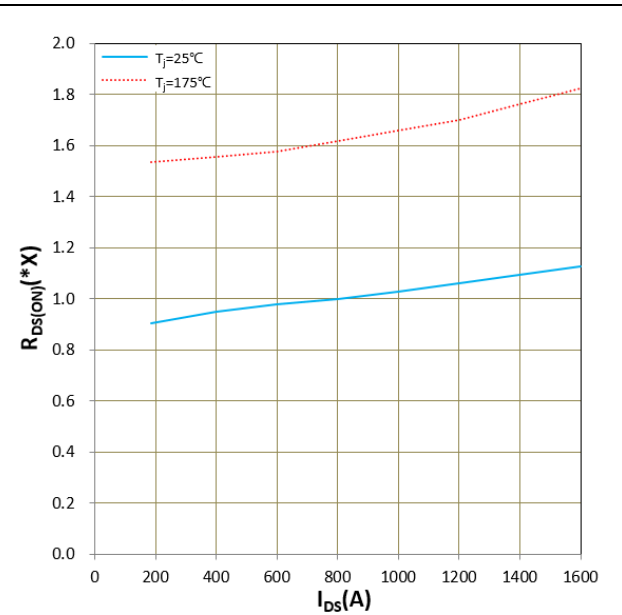
Figure 11. R_{DS(ON)} vs I_{DS} 1.0x = 2.1\text{m}\Omega
