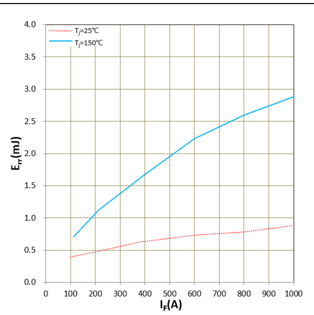
Figure 19. E rr vs I F V DD =600V, R G =2.2Ω, V GS =+15V/-4V Inductive Load
