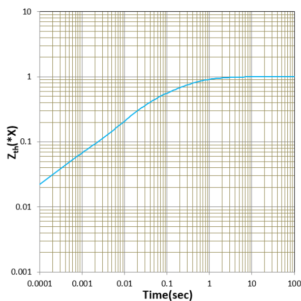
Figure 23. Transient thermal impedance 1.0x = 0.156\text{K/W}
