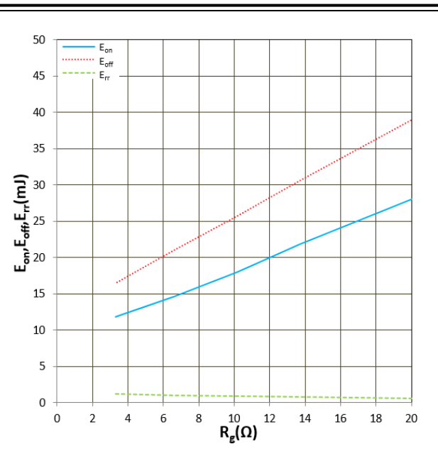
Figure 17. E_{on} , E_{off} , E_{rr} vs R_g T_j = 150^\circ\text{C} , V_{CC} = 600\text{V} , I_D = 400\text{A} , V_{GS} = +15\text{V}/-4\text{V} Inductive Load
