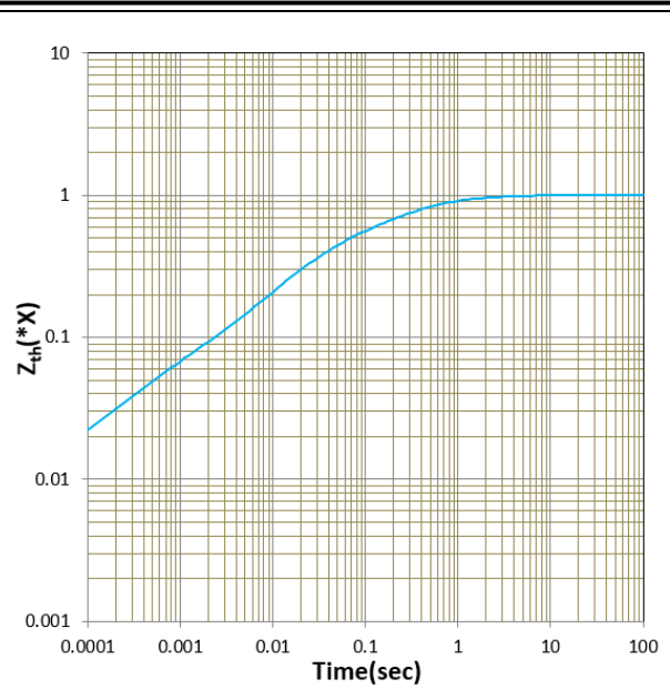
Figure 21. Transient thermal impedance 1.0x = 0.156K/W
